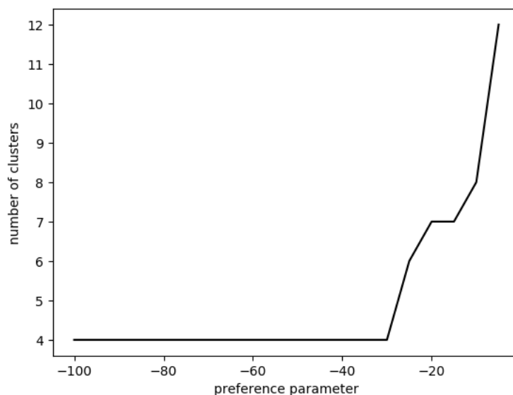
Figure 6 - Number of clusters derived from affiliation propagation versus shared preference (best three indicators only)
