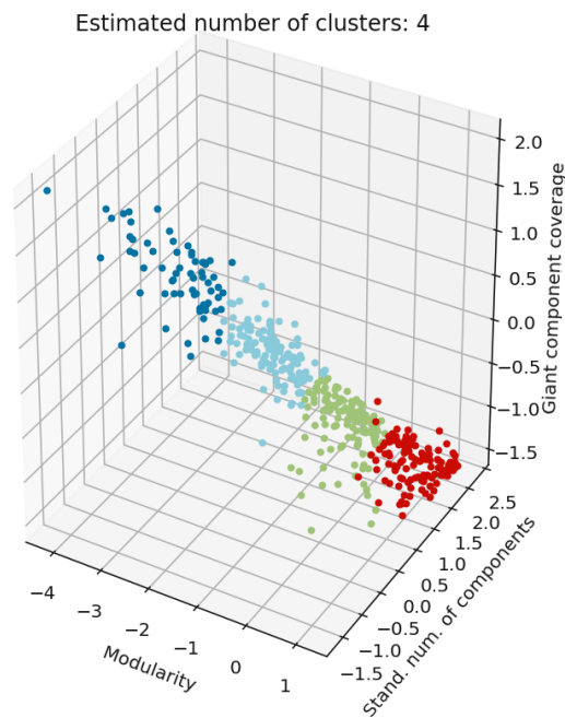
Figure 8 - 3D representation of the resulting clusters. Note that figure 7 is the 2D view from above.
