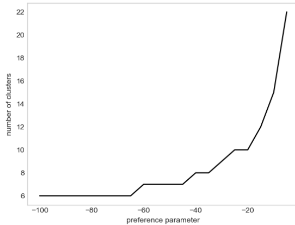
Figure 4 - Number of clusters derived from affiliation propagation versus shared preference (all indicators included)
