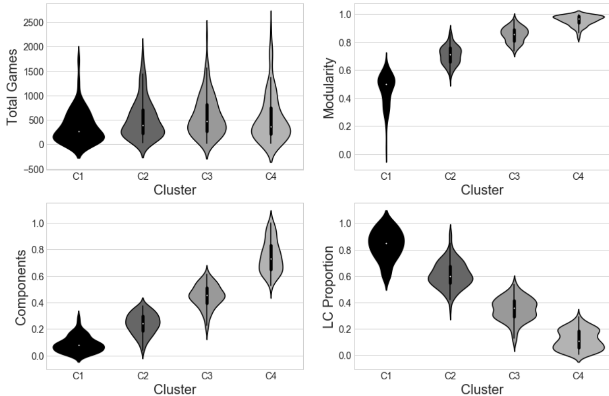
Figure 9 - Violin plots for total games, modularity, components and largest component proportion per cluster
