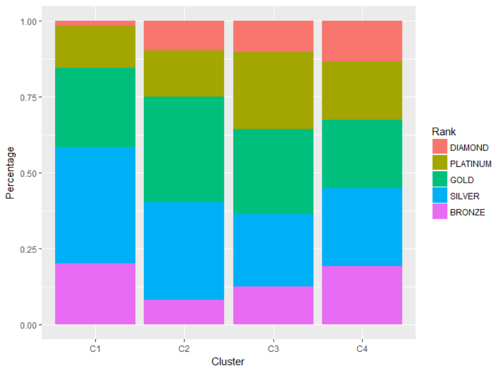
Figure 11 - Rank distribution per cluster. C1 has less high ranked players than other clusters. C3 and C4 are disproportionately higher ranked.
