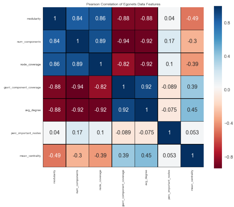
Figure 3 - Bivariate correlations between variables of interest.
