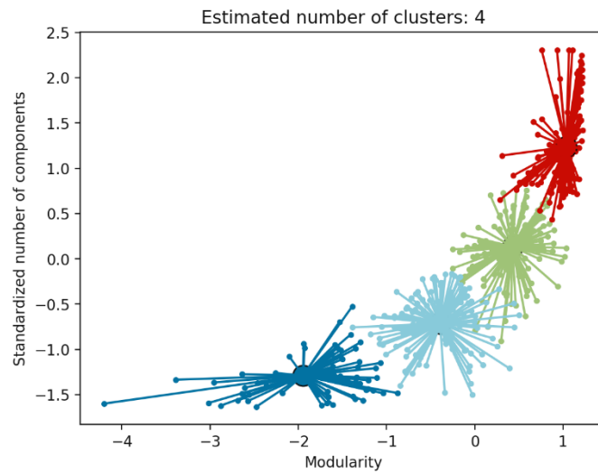
Figure 7 - Graphical representation of clusters resulting from the affiliation propagation algorithm with preference -30 and restricted to the best three indicators. This is a 2D slice of the 3D space.
