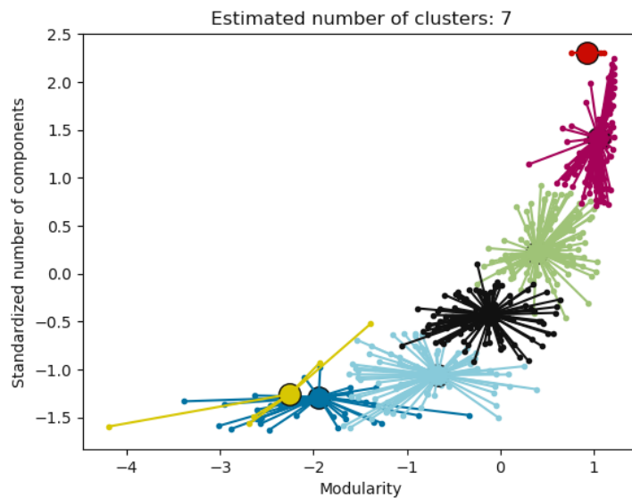
Figure 5 - Graphical representation of clusters resulting from the affiliation propagation algorithm with preference -45 and all indicators included. This is only a 2D slice of a 7 dimension space for illustration purposes.
