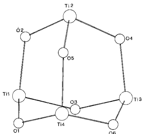
Fig. 9. Drawing of the \text{Ti}_4\text{O}_6 core of 21 ( \text{Cp}^* rings omitted for clarity).
