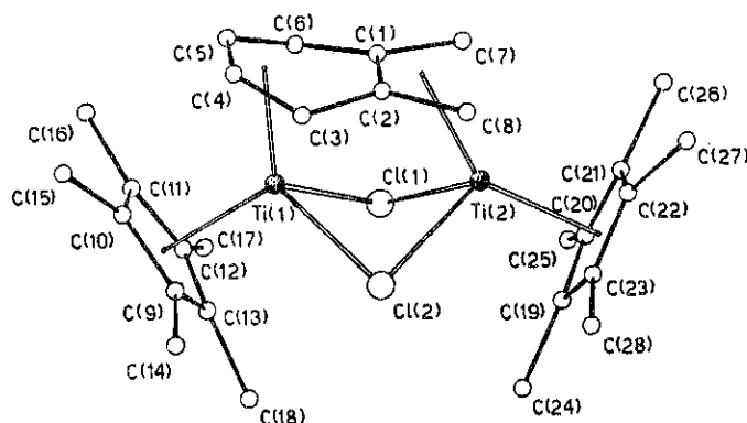
Fig. 4. View of the structure of 12 .
