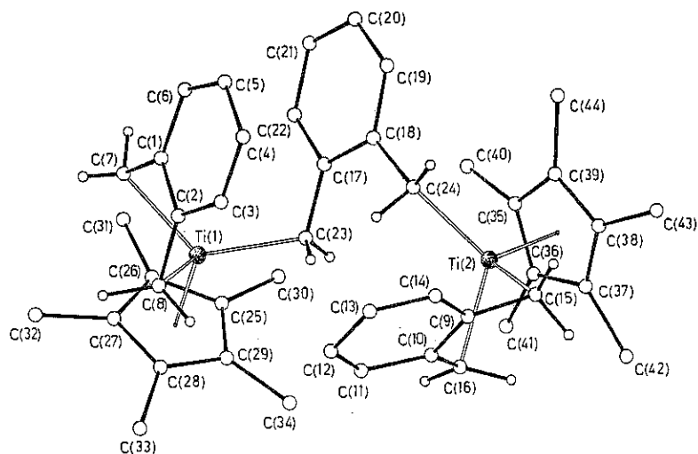
Fig. 2. View of the structure of 11 .
