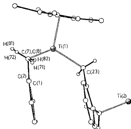
Fig. 3. Projection of a part of the structure of 11 along the line through C(7) and C(8).
