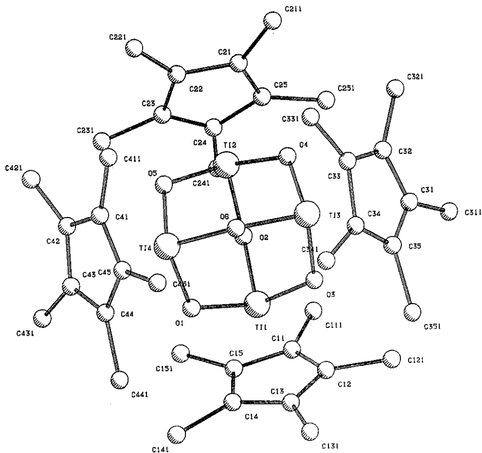
Fig. 8. View of the structure of 21 .
