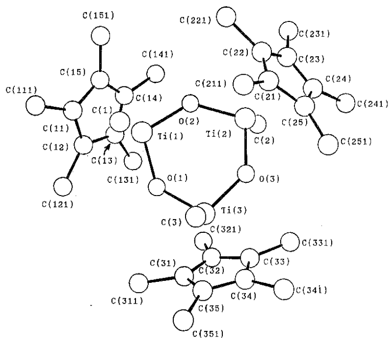
Fig. 6. View of the structure of 23 .
