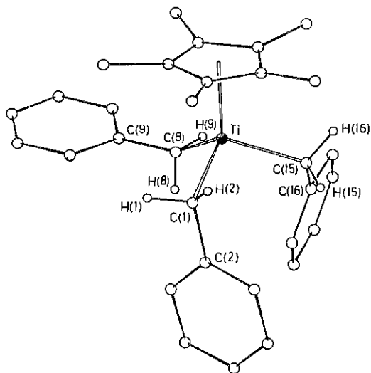
Fig. 1. View of the structure of 5 .
