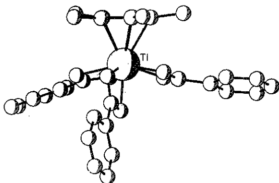
Fig. 11. View of the structure of 29 .
