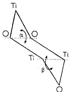
Fig. 10. \text{Ti}_3\text{O}_3 chair ring of 21 showing the \alpha and \beta angles.
