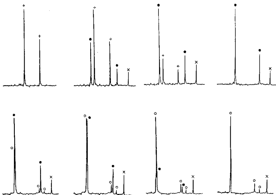
Fig. 5. ^1\text{H-NMR} ( \text{C}_6\text{D}_6 ) sequential study corresponding to Scheme 5 + 7; \bullet 22 ; \circ 23 ; \times \text{CH}_4 .
