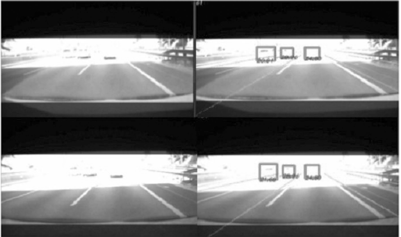
Fig. 13. Cars remain under tracking in spite of bad image conditions.
