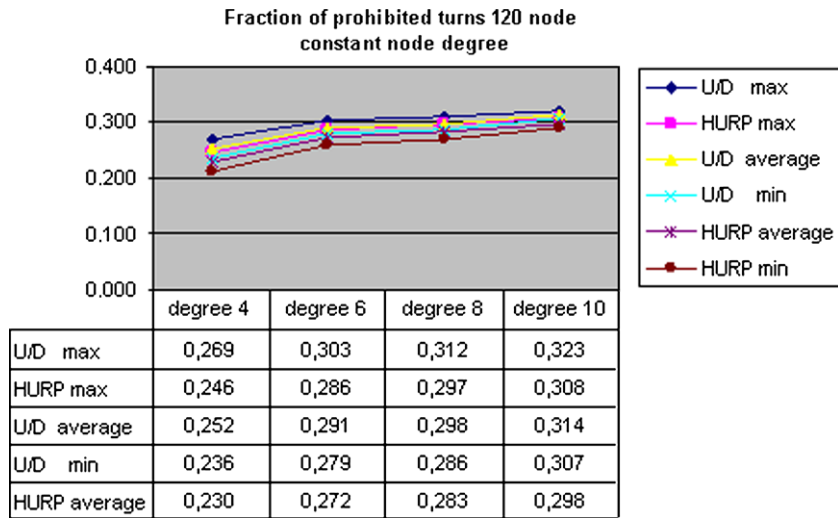
Fig. 9. Fraction of prohibited turns as a function of node degree. All nodes at each topology have same degree.
