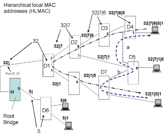
Fig. 3. Assignment of Hierarchical Local MAC addresses based on spanning tree. -.-Tree forwarding. —Transversal forwarding.
