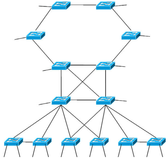
Fig. 11. Metro topology.
