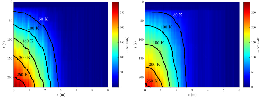
Fig. 7. Heating z-t map obtained when the pump is turned on (at t = 15-20 s, P_{\text{pump}} \approx 105 mW): Left: on-resonance; Right: off-resonance.
