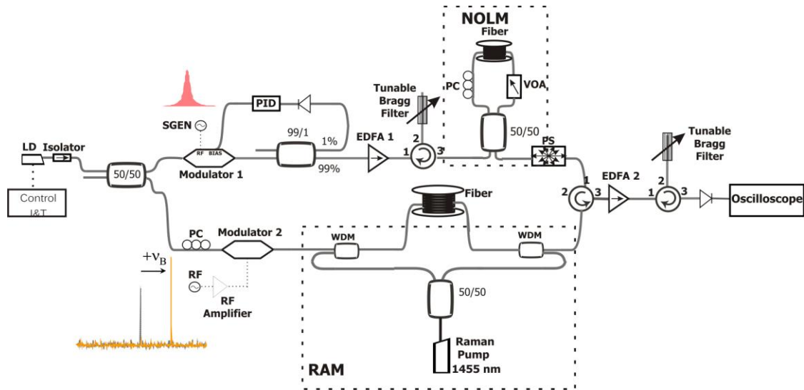
Fig. 1. Experimental setup of the Raman-assisted distributed Brillouin sensor. LD: Laser Diode; PC: Polarization controller; SGEN: Pulse generator; PID: Proportional-Integral electronic circuit; EDFA: Erbium Doped Fiber Amplifier; RF: Radio-Frequency generator; NOLM: Non-linear Optical Loop Mirror; PS: Polarization Scrambler; WDM: Wavelength Division Multiplexer.
