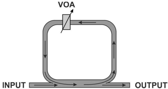
Fig. 1. Fiber-based lossy ring resonator considered.
