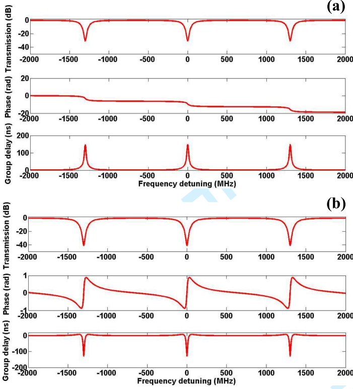
Fig. 2. Phase, modulus and group delay response vs. frequency in a 1.59 meter and \kappa=0.7 ( \approx 1.55 dB) fiber loop with (a) 1 dB attenuation and (b) 2 dB attenuation.
