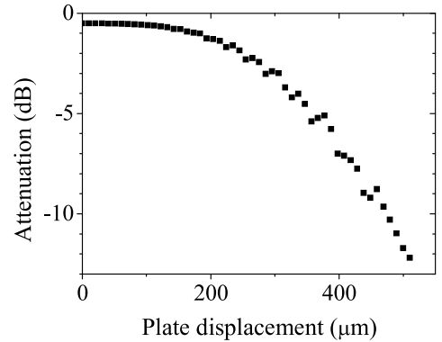
Fig. 4. Attenuation profile of the bending plates versus the displacement.
