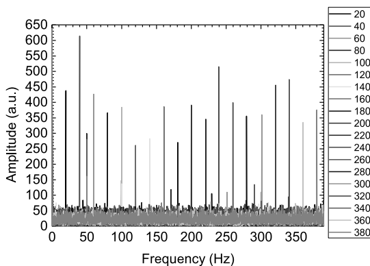
Fig. 5 FFT spectra of the optical power variation of the \phi OTDR signal for consecutive traces in the point of the FUT with minimum signal for applied frequencies between 20 Hz and 380 Hz, using the same conditions of fig. 4.
