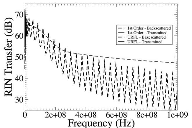
Fig. 2 RIN transfer functions from URFL (black) and first-order (red) pumps to the transmitted (solid) and backscattered (dashed) signals in a 125 km span. First-order pump
