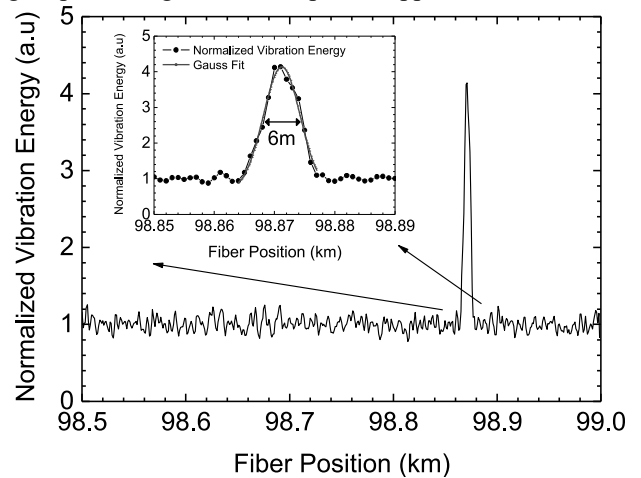
Fig. 6 Normalized energy density of vibrations around 20 Hz along the FUT when a vibration of 20 Hz was applied to the PVC tube (at \approx 98.8 km). The normalized vibration energy density of the frequencies around 20 Hz was calculated for each fiber position as the RMS of the interval 18-22Hz (signal) divided by the RMS of the interval 350Hz-390Hz (noise) of the FFT of the optical power variation of the \phi OTDR signal. In the inset figure a gaussian fit of the points where the vibration was detected is shown, presenting 6m at FWHM.
