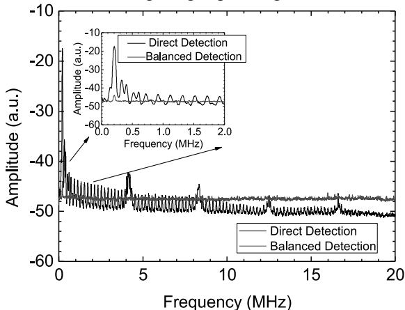
Fig. 3 Characterization of the noise in the electrical spectrum domain of the signal returning from the fiber when a Raman pump power of 28.5 dBm is launched on both ends of the FUT without input \phi OTDR pump using balanced and direct detection. While balanced detection only presents white noise and a small peak at 0.2 MHz, the direct detection presents higher noise levels and periodical structure with peaks every 0.2 MHz.
