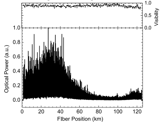
Fig. 4 \phi OTDR interference signal along the FUT when the Raman pump power launched on each end of the FUT was 28.5 dBm. In this case, the \phi OTDR pump power was chosen as the one ensuring the best performance. The top figure shows the visibility of the interference signal, computed as V=(T_{\max}-T_{\min})/(T_{\max}+T_{\min}) where T_{\max} and T_{\min} are the maximum and minimum values of the trace over a window of 500 m.
