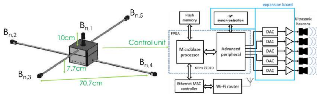
Figure 2. General description of the LOCATE-US beacon unit.
