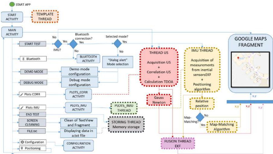
Figure 12. LOCATE-US Application flowchart.
