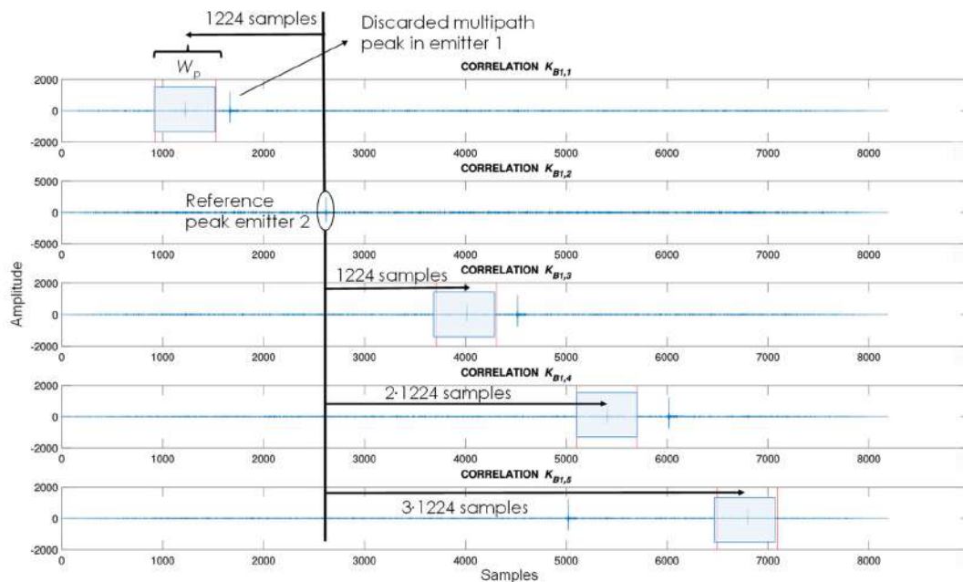
Figure 9. Example of correlation functions from the U-LPS 1 with TDOA \neq 0 .
