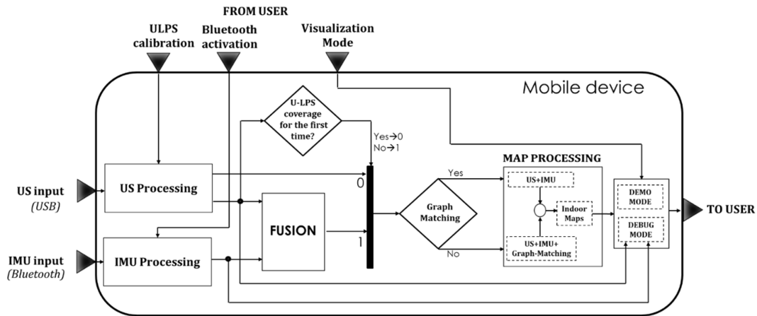
Figure 6. Block diagram of the LOCATE-US application.
