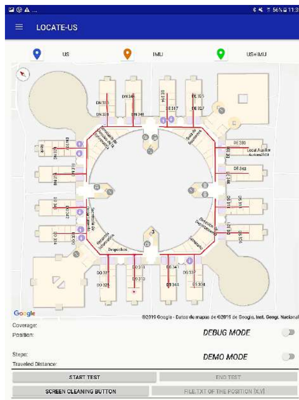
Figure 5. Graph considered in the LOCATE-US application for the corridors of the third floor from the School of Engineering in the University of Alcalá.
