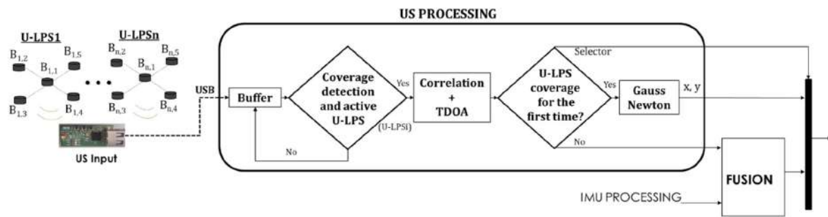
Figure 7. Block diagram of the US Processing tasks.
