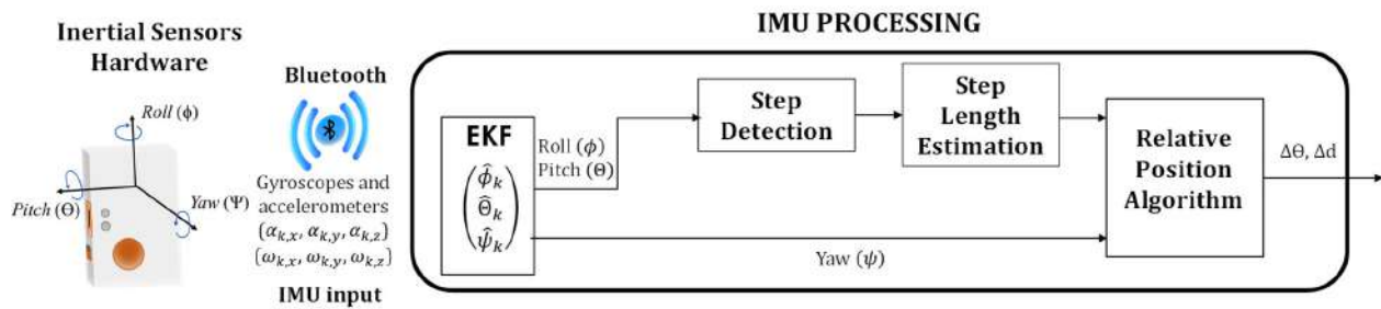
Figure 10. Block diagram of the inertial measurement unit (IMU) processing tasks.
