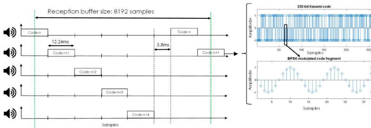
Figure 4. Modulation scheme and medium access technique applied to the beacon transmissions.
