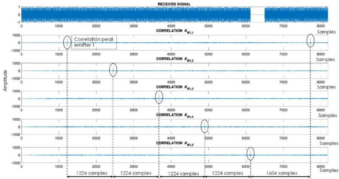
Figure 8. Example of correlation functions for U-LPS 1 when the receiver's position is equidistant to all emitters (TDOA = 0).
