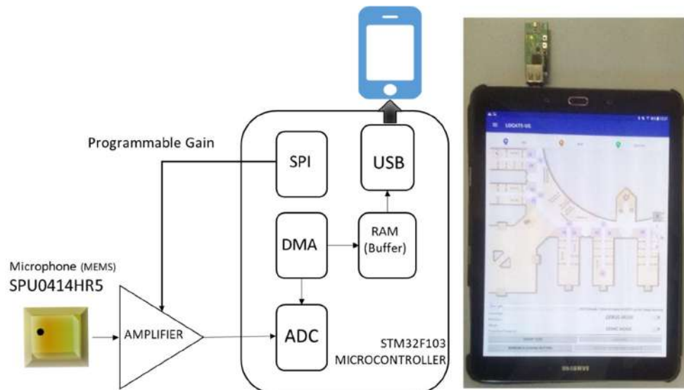
Figure 3. Block diagram and view of the acquisition module for LOCATE-US.
