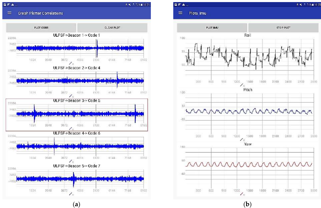
Figure 16. Additional screens in DEBUG mode. (a) US correlations, (b) IMU raw data.
