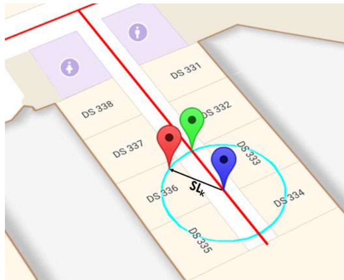
Figure 11. Example of graph-matching. The blue marker denotes the previous position, the red marker the new estimated one from the IMU sensors, and the green marker the one corrected by graph-matching.
