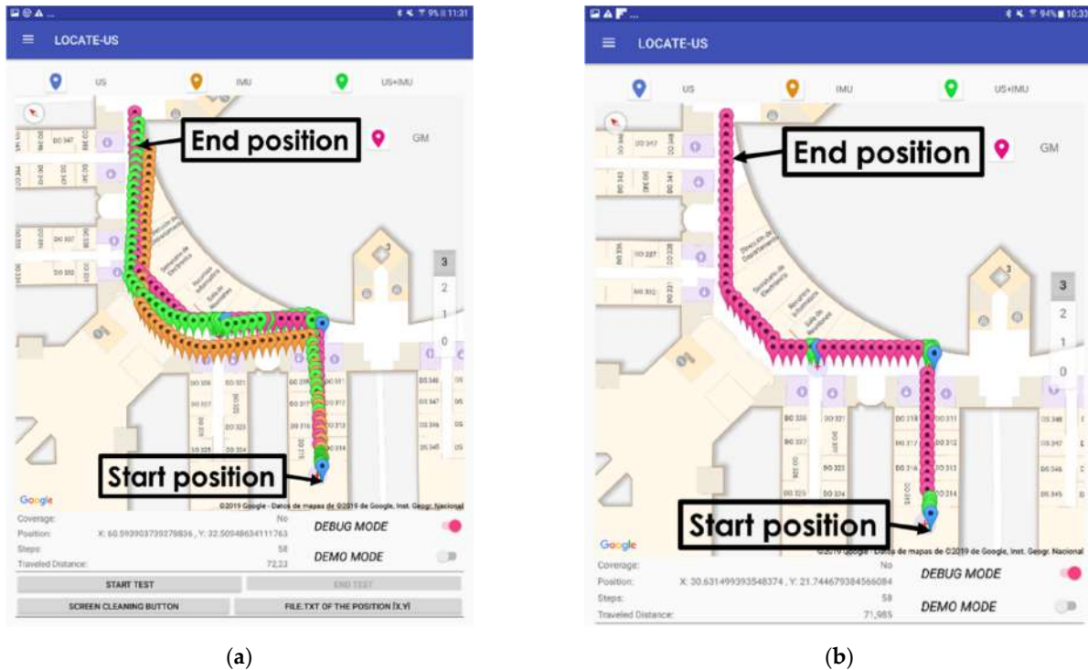
Figure 21. Android screenshots of the experimental test which includes the graph-matching technique. (a) Fusion (US+IMU), US, IMU and GM; (b) Fusion (US), US and GM.
