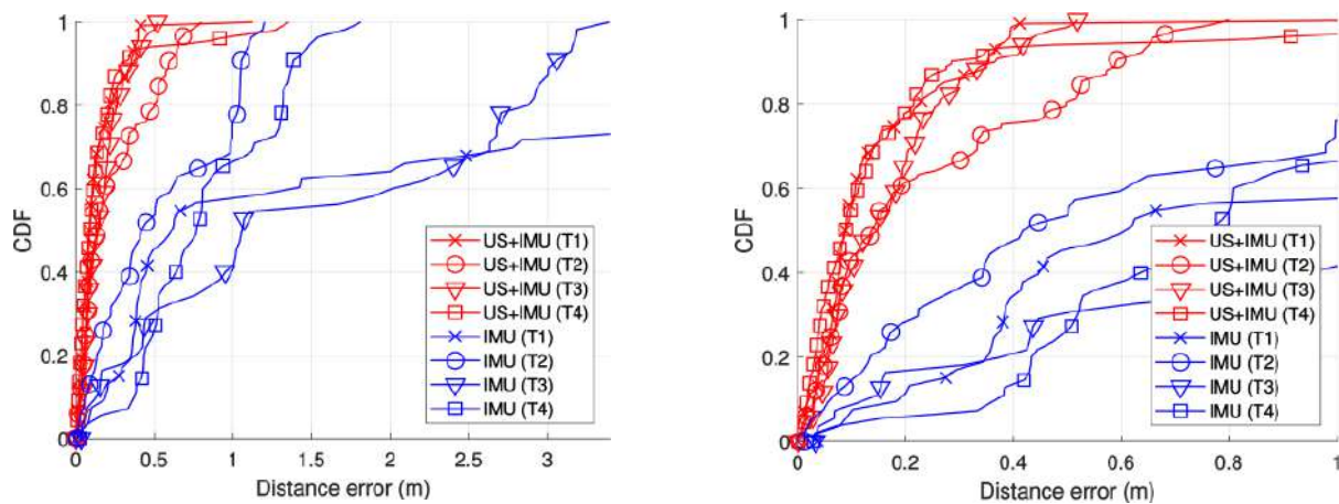
Figure 20. Cumulative distribution functions (CDFs) of distance errors related to the four experimental tests (left), comparing the IMU and the fusion (US + IMU) results, as well as a zoom for a distance error of 1m (right).
