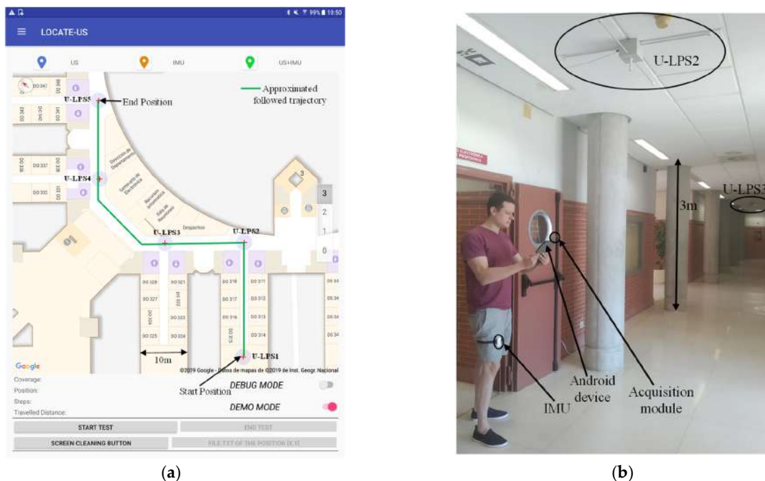
Figure 18. (a) Indoor map with the U-LPS positions and the trajectory followed by the user (in the real experiments users try to carefully follow it). (b) General view of the experimental setup with a person equipped with an Android device connected to the acquisition module and the IMU installed outside the pocket of the user.
