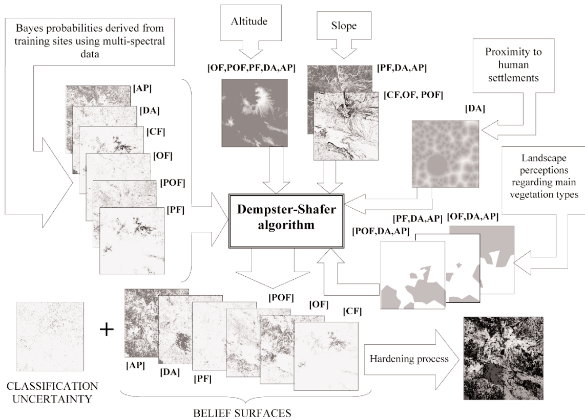
Figure 3.2. Dempster-Shafer classification allows combine different lines of evidences derived from satellite imagery and expert knowledge to produce a set of layers (belief surfaces) that define the probability of each pixel belonging to each of the classification categories. In addition a layer showing the uncertainty associated to the classification process is generated.
