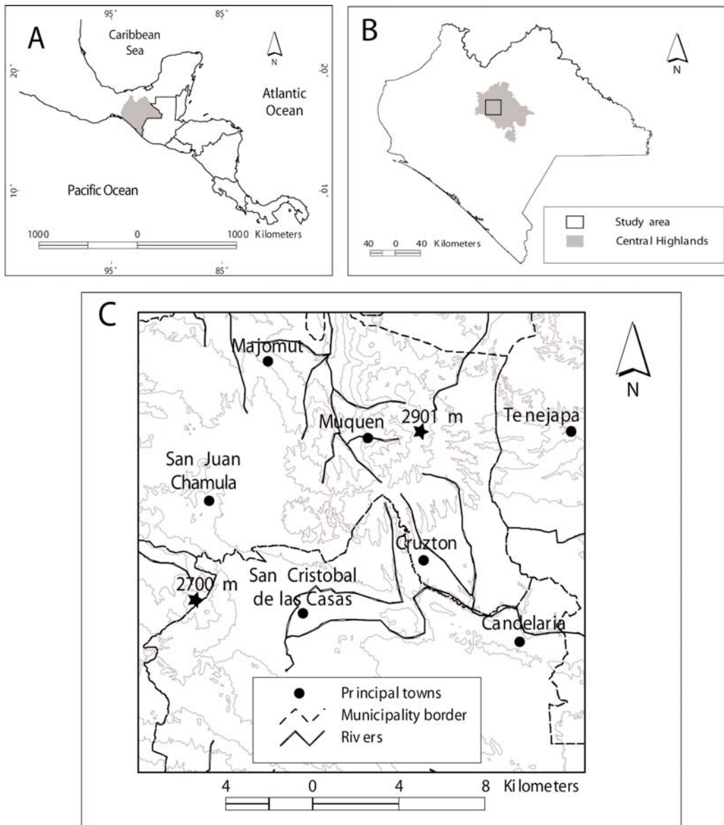
Figure 3.1. (A) The state of Chiapas, southern Mexico, and northern Central America. (B) Geographical allocation of the highlands of Chiapas and the central Highlands within the state. (C) Characteristics of the study area: municipalities, rivers, principal towns and topographical features.
