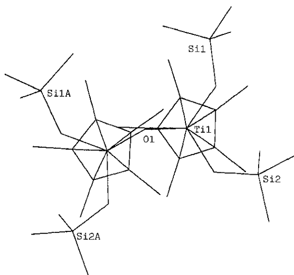
Fig. 2. Projection of the molecule of 5 on the \text{Cp}^* plane.
