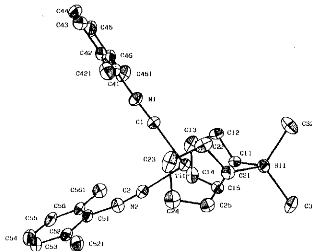
Fig. 1. ORTEP view of [\text{Ti}\{\text{Me}_2\text{Si}(\text{C}_5\text{H}_4)_2\}\{\text{CN}(2,6\text{-Me}_2\text{C}_6\text{H}_3)_2\}] ( 3 ) with atom labelling scheme.
