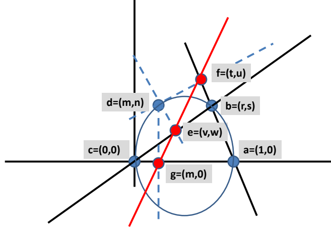
Figure 1: Illustration of Simson's Theorem
