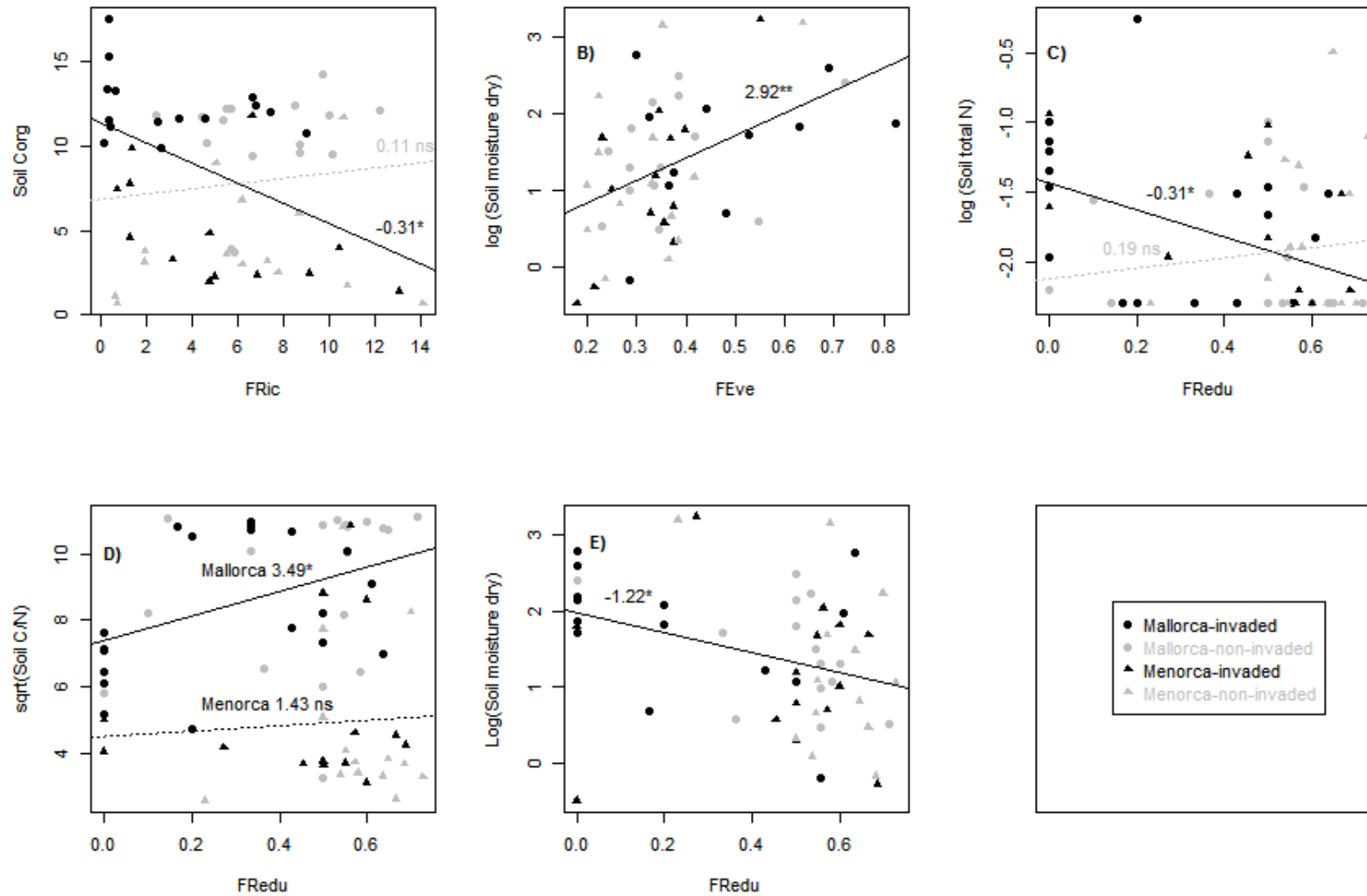
Figure 2. Relationship between functional indexes and ecosystem properties. Lines show the adjustment between variables and the coefficient of the functional index in a linear model with the ecosystem property as dependent variable and the functional property, island and invaded status as fix factors (all coefficients are shown in Table 2). Two lines are shown in the same graph when there was a significant interaction between the functional index and invaded status (black and grey lines for invaded and non-invaded plots respectively) or between the functional index and the island. Significance: *** p \leq 0.001 , ** 0.01 \geq p > 0.001 , * 0.05 \geq p > 0.01 , + 0.1 \geq p > 0.05 , ns p > 0.01 .
