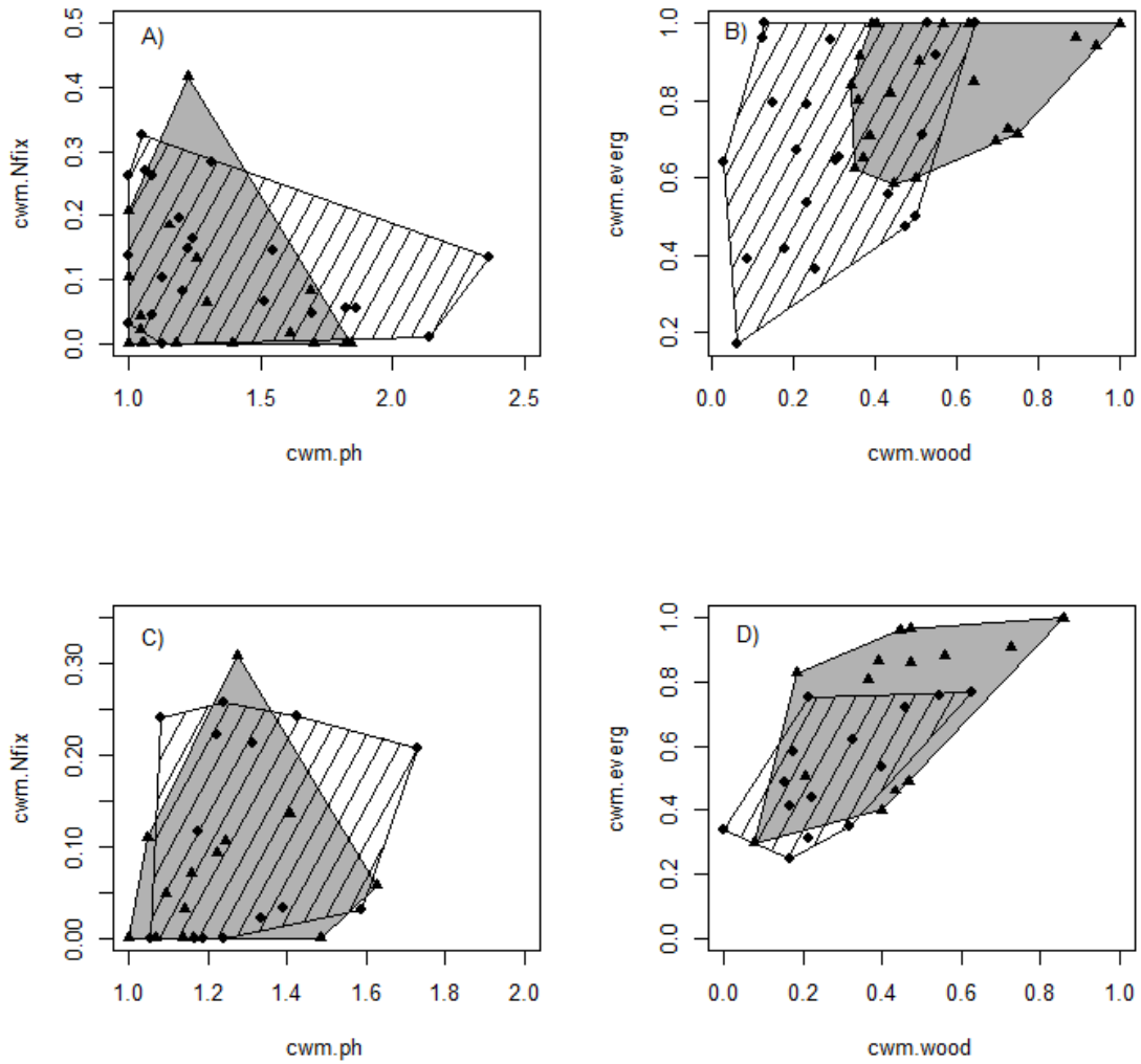
Figure 1. Functional spaces occupied by communities. Dotcharts showing the position of Carpobrotus invaded (triangles) and non-invaded plots (diamonds) in the space defined by the community weighed means (CWM) of plant height and N-fixation (A, C) and by the CWMs of woodiness and evergreenes (B, D). A, B- Mallorca, C, D – Menorca. CWMs of invaded plots were calculated including Carpobrotus . The grey and lined areas include all invaded and non-invaded plots, respectively.
