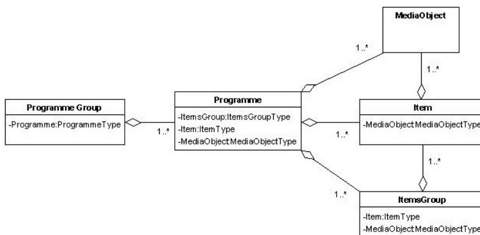
Figura 36 - The P_Meta Model 97
